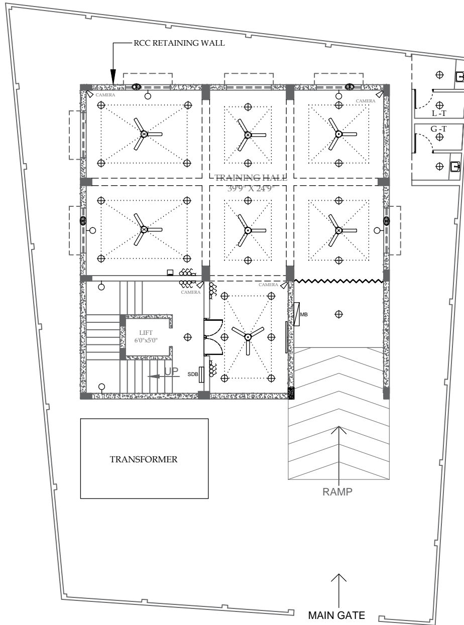
CELLAR FLOOR PLAN
