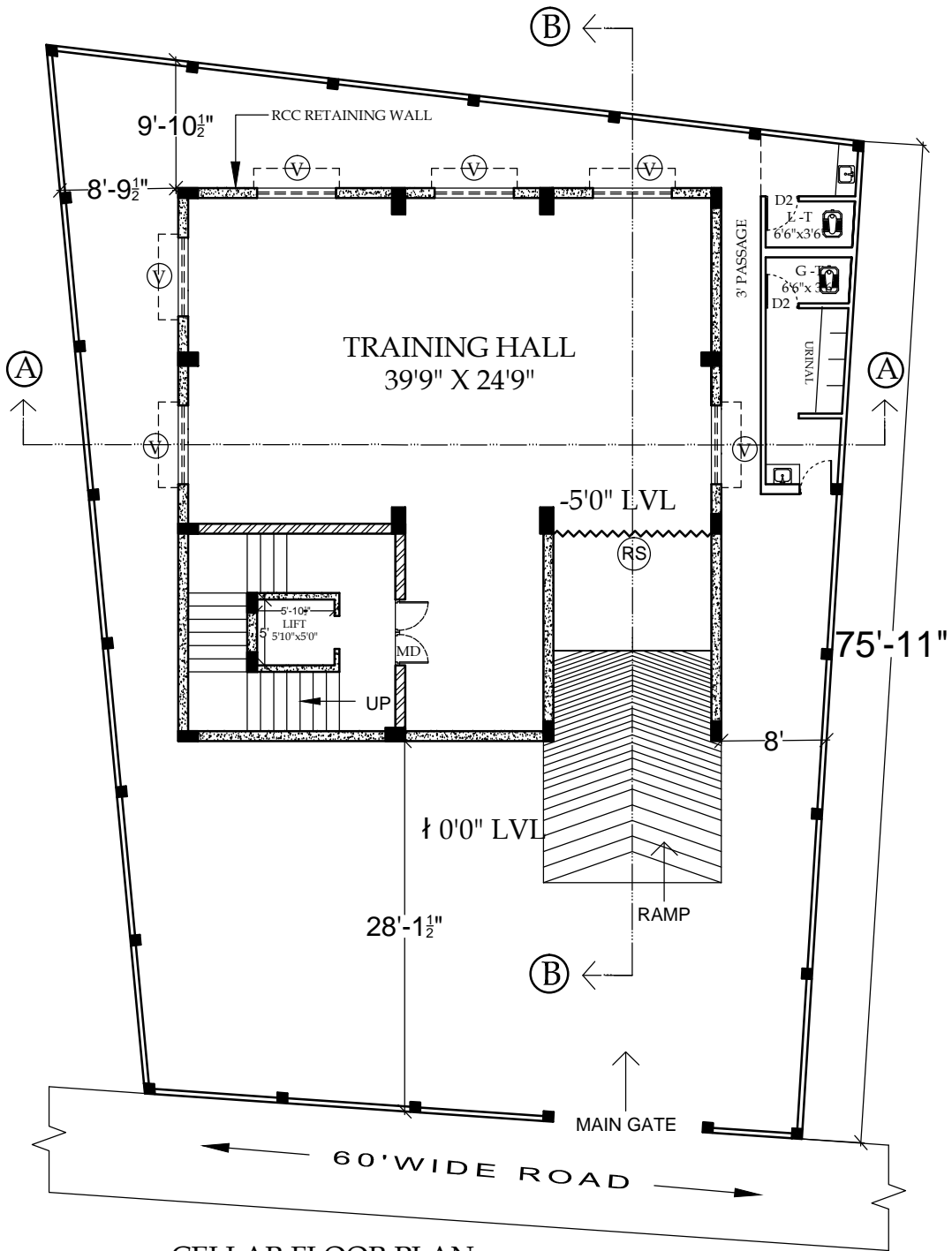
CELLAR FLOOR PLAN
